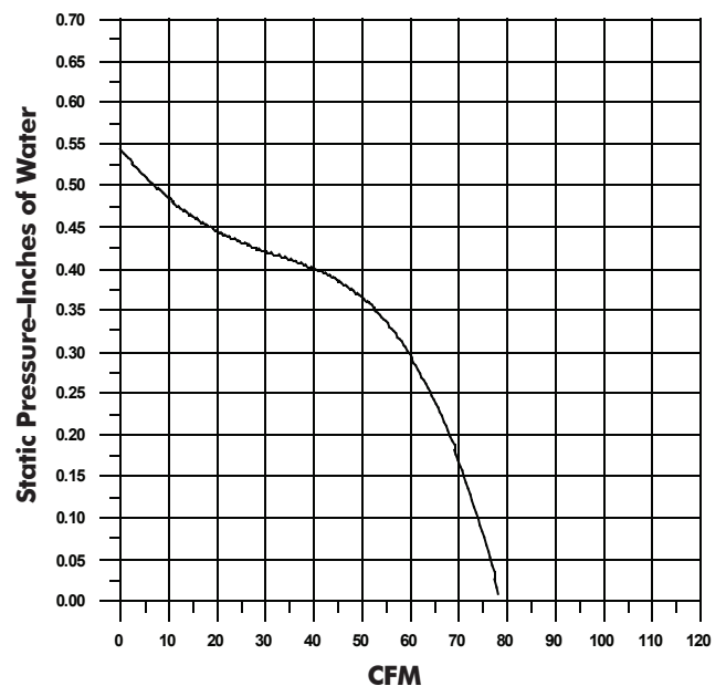
NuVent Product Performance Model NXMR70L
